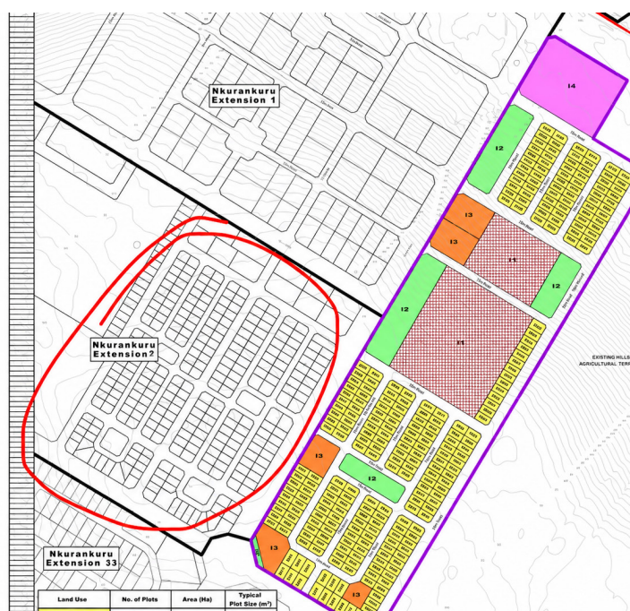
Indicative Nkurenkuru Extension 7 housing-development layout
